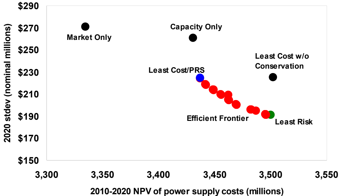
Figure 3: Efficient Frontier
